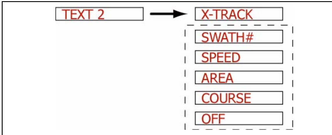
Figure 25: Selecting the Text 2 Message
