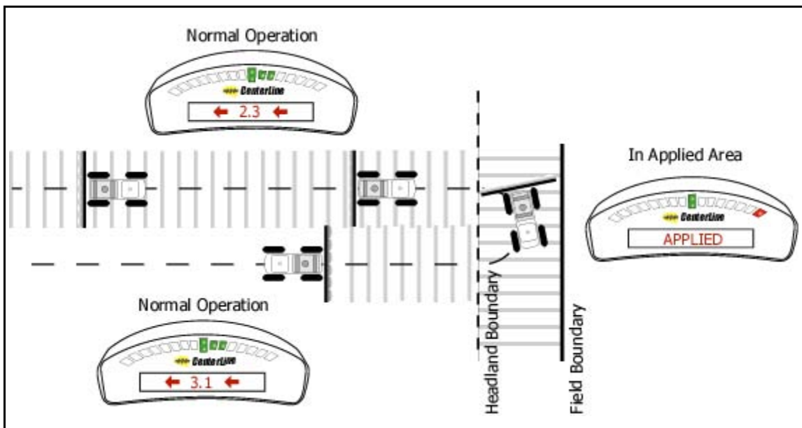
Figure 49: Applied Area Detection in Headlands
