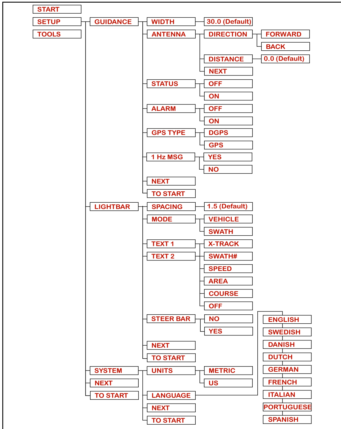
Figure 30: CenterLine Setup Flow Diagram
