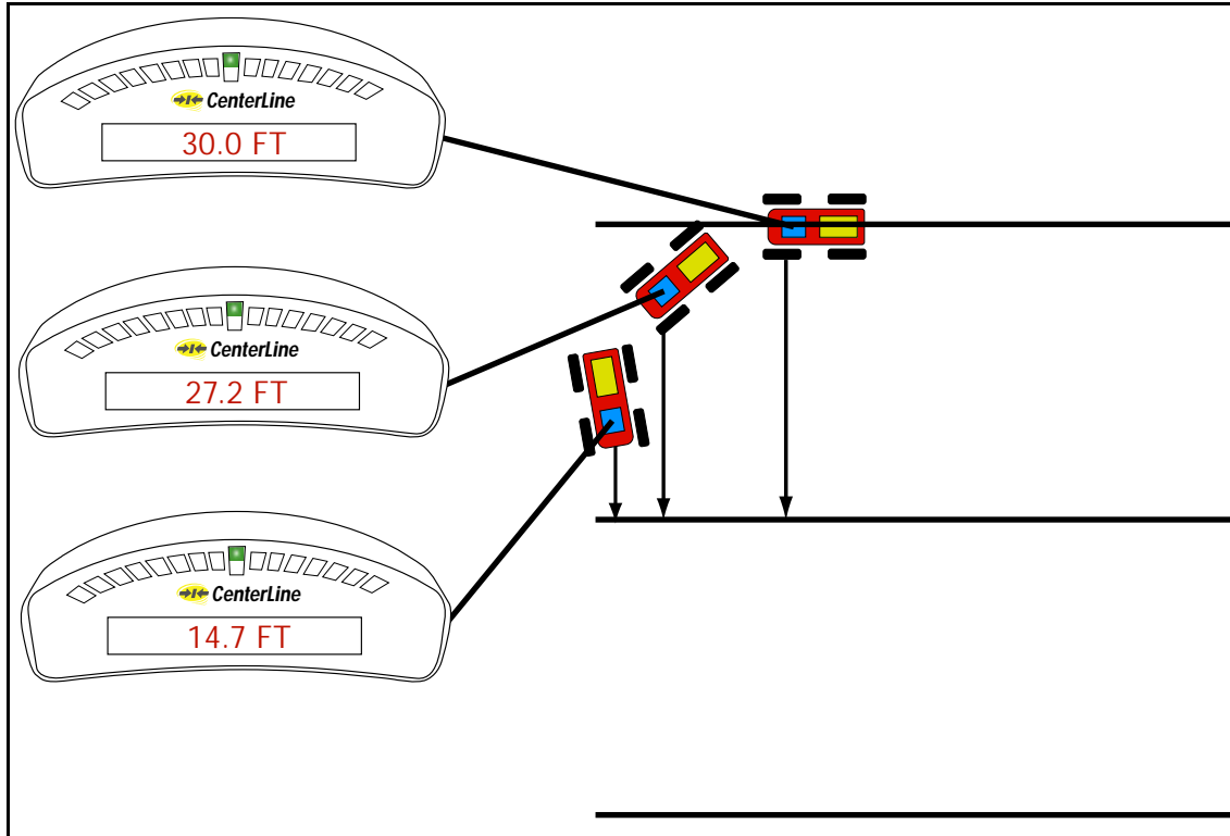
Figure 45: Distance to Next Straight Swath
