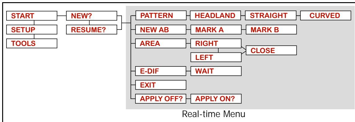
Figure 32: Real-Time Operation Flow Diagram
